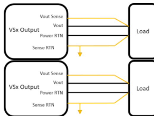
Figure 4: M4054 Sense line connection
